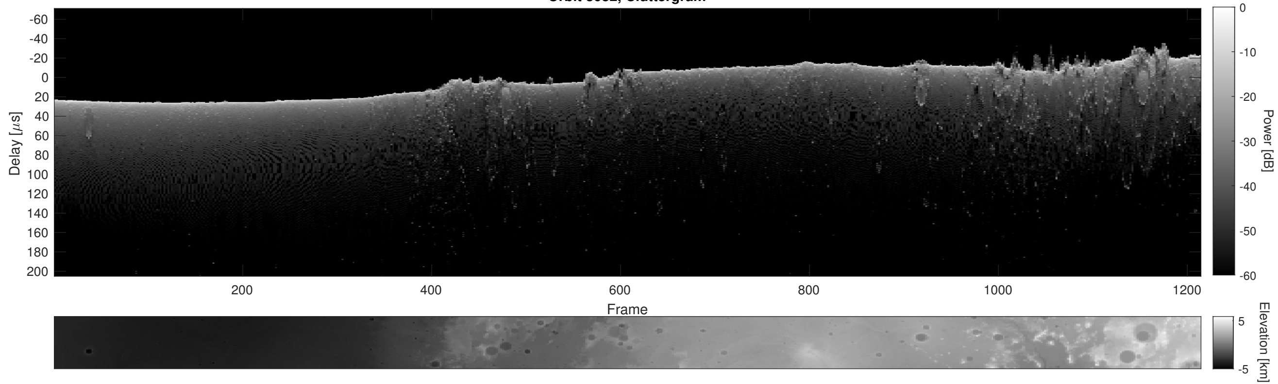
Orbit 3032, Cluttergram
