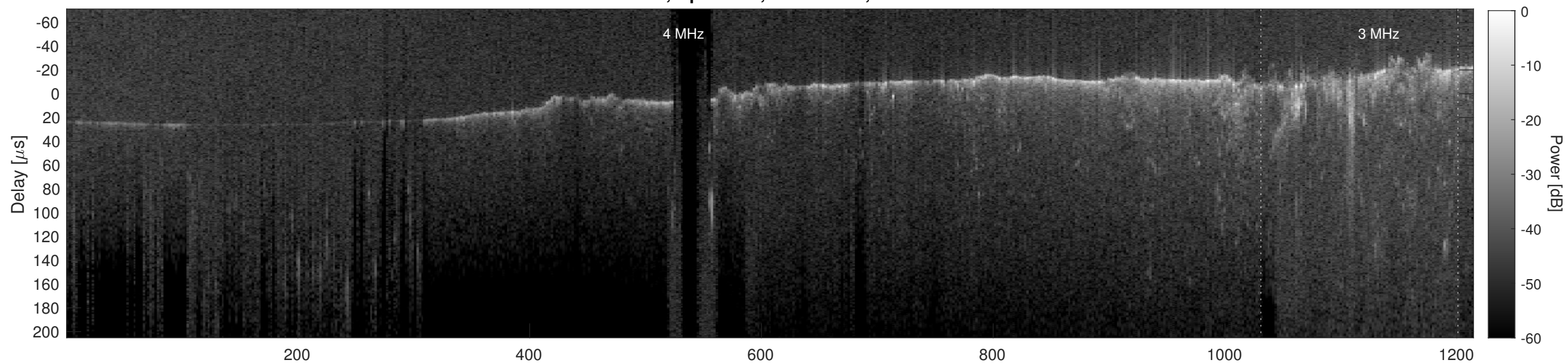
Orbit 3032, Cluttergram
