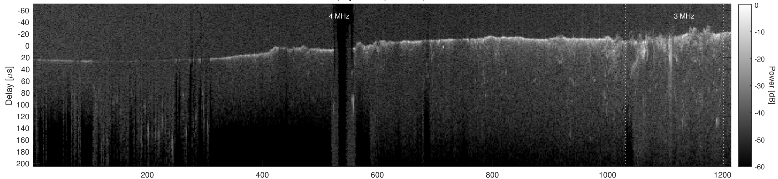
Orbit 3032, Cluttergram
