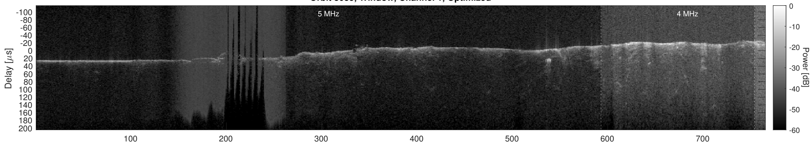
Orbit 3035, Cluttergram
