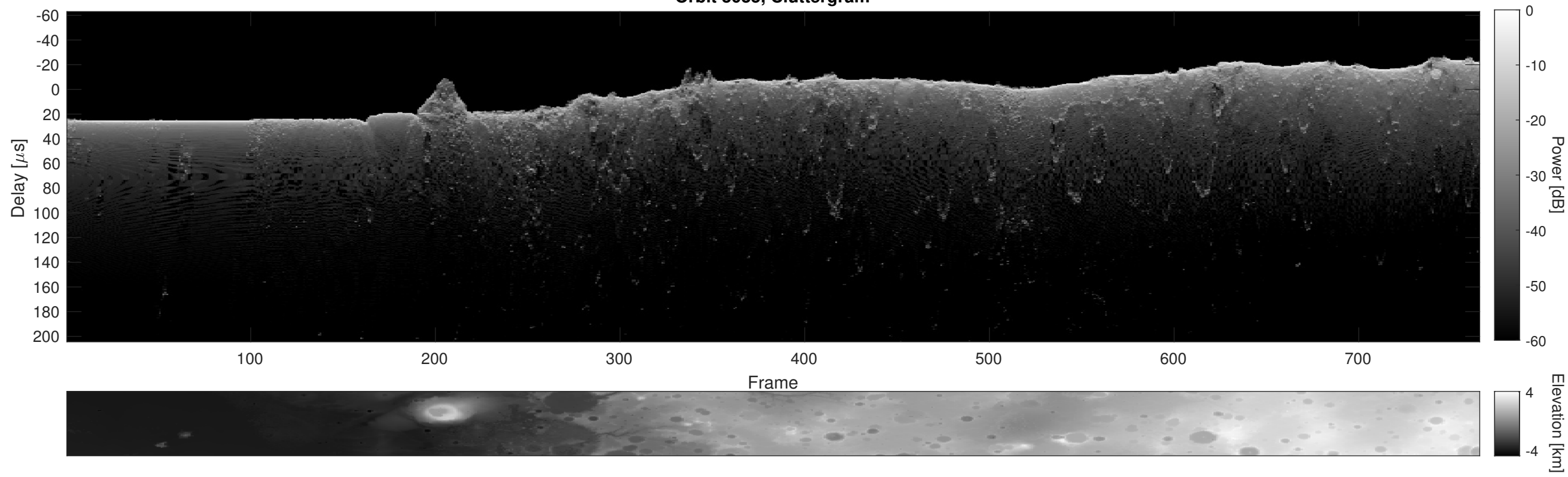
Orbit 3035, Cluttergram
