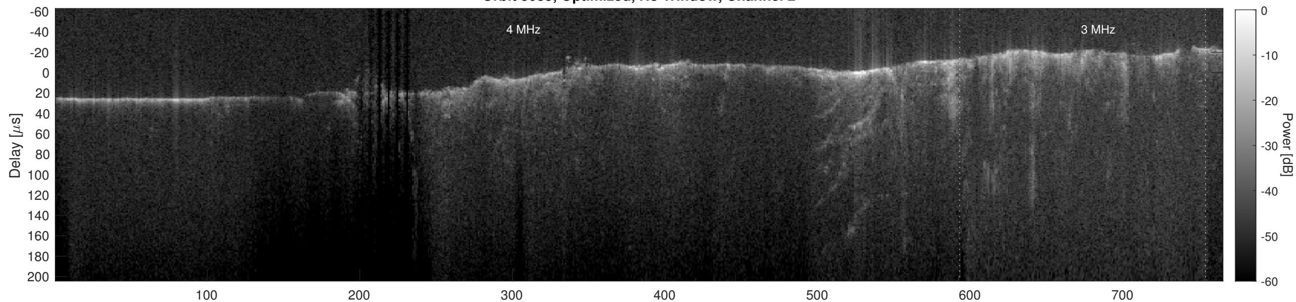
Orbit 3035, Cluttergram
