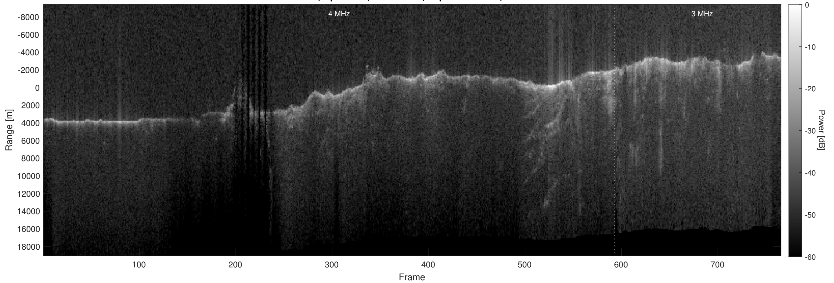
Orbit 3035, Optimized, No Window, Depth-Corrected, Channel 2
