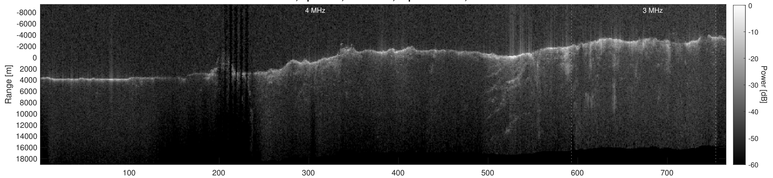
Orbit 3035, Depth-Corrected Cluttergram
