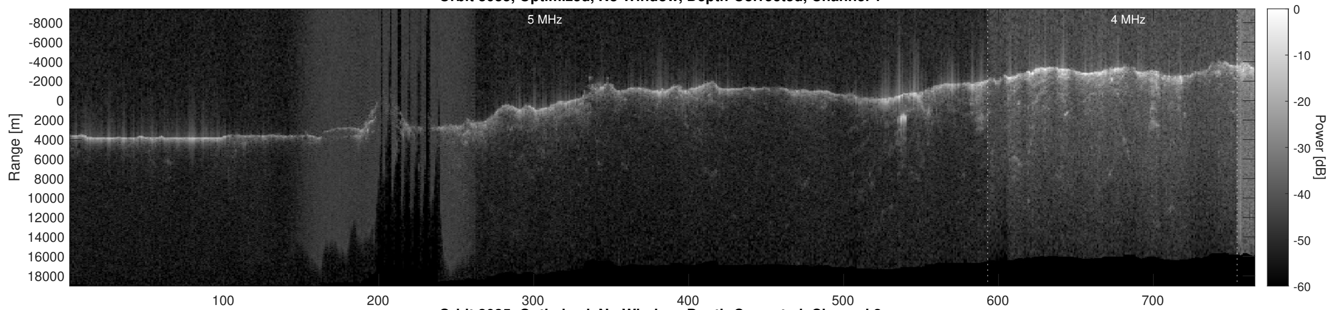
Orbit 3035, Optimized, No Window, Depth-Corrected, Channel 2
