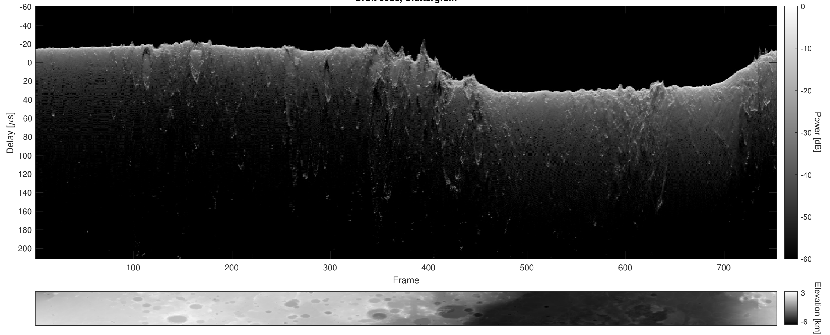
Orbit 3036, Cluttergram
