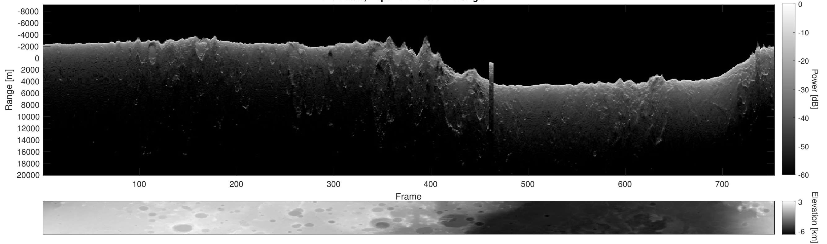
Orbit 3036, Depth-Corrected Cluttergram
