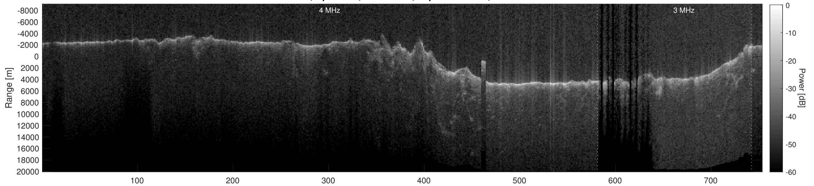
Orbit 3036, Depth-Corrected Cluttergram
