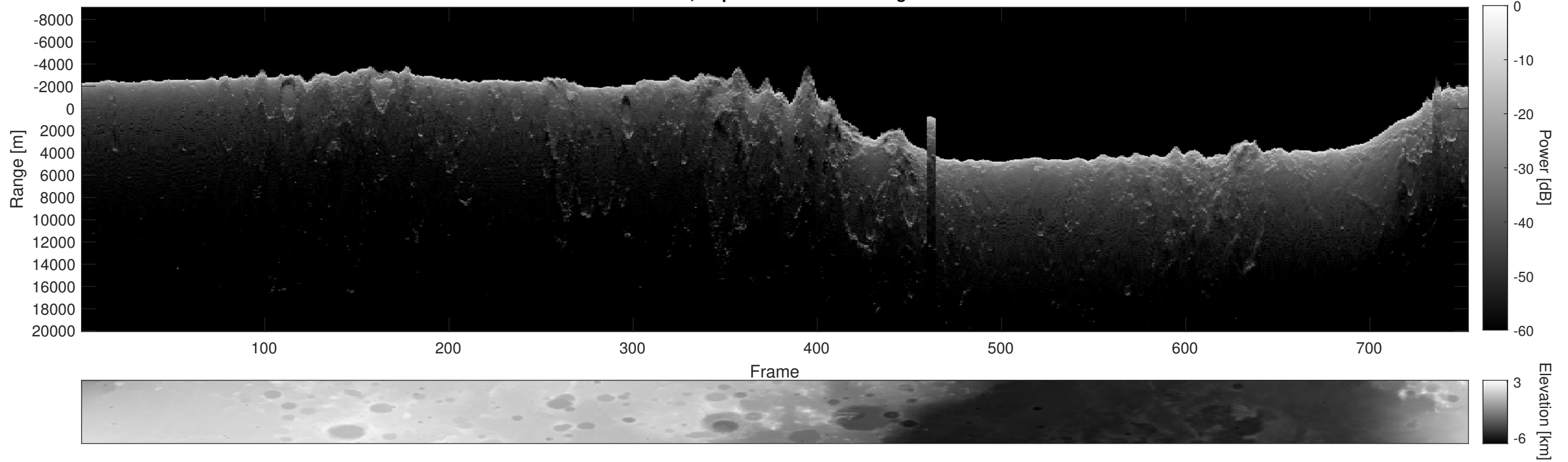
Orbit 3036, Depth-Corrected Cluttergram
