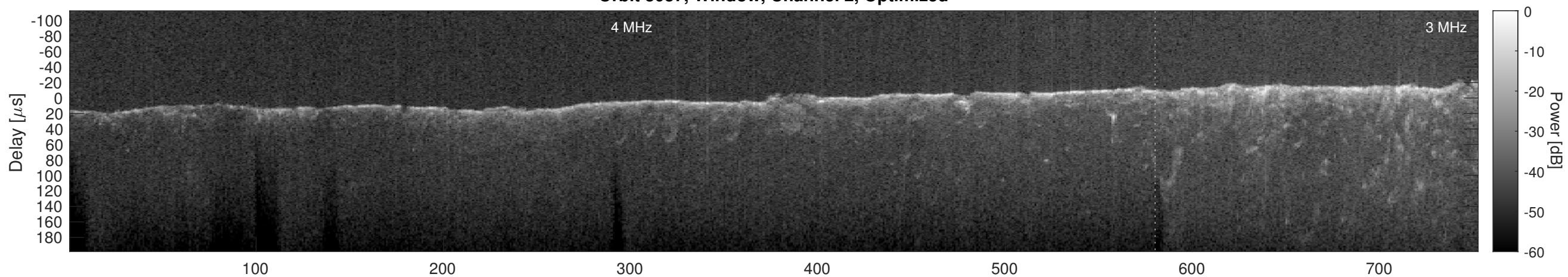
Orbit 3037, Cluttergram
