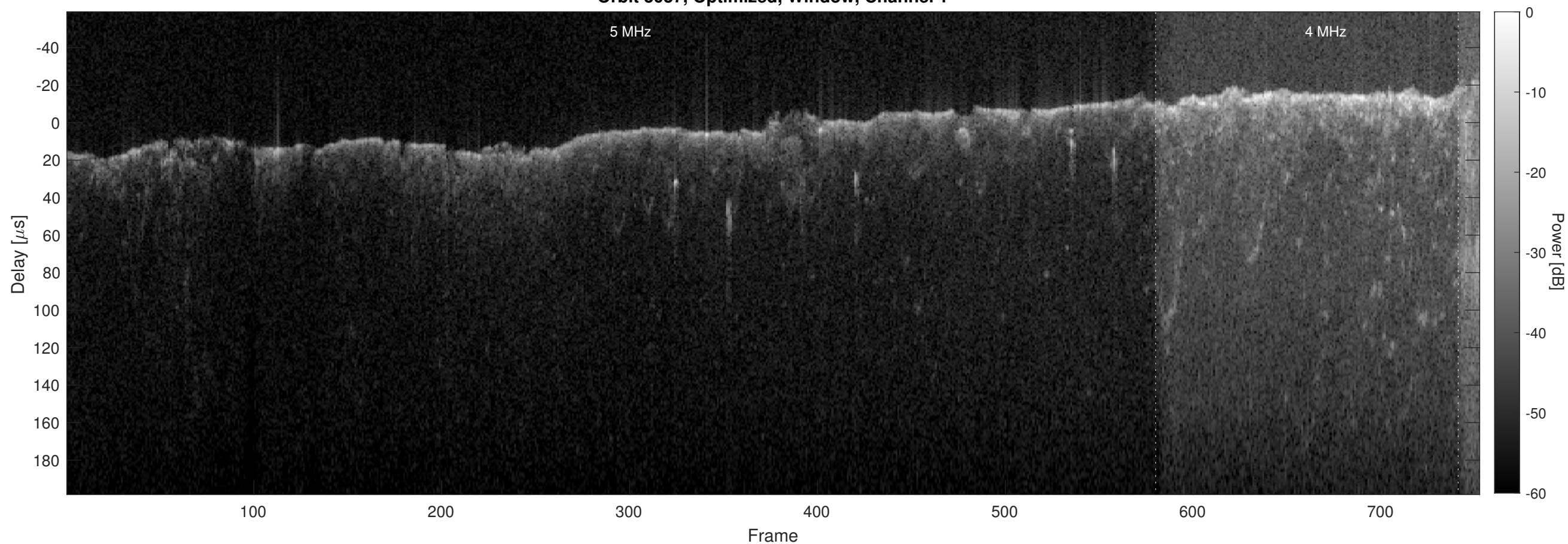
Orbit 3037, Optimized, Window, Channel 2
