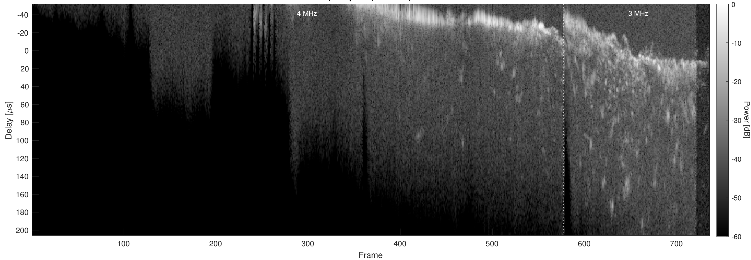
Orbit 3041, Chapman, Window, Channel 2
