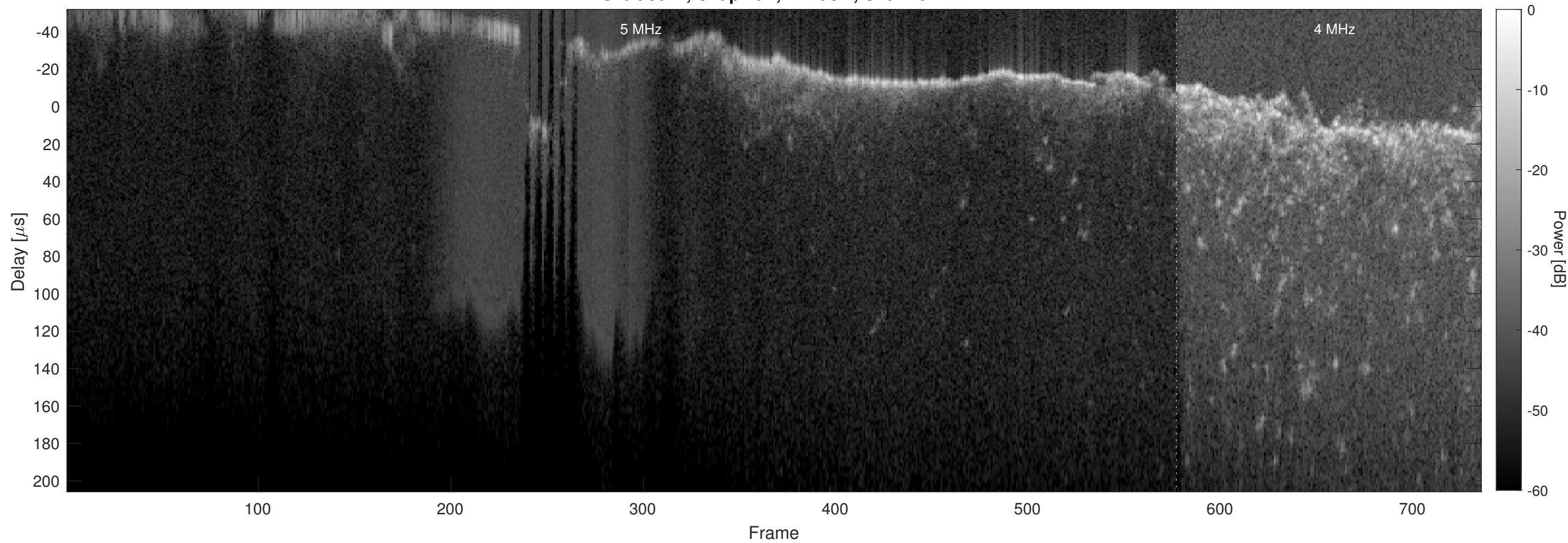
Orbit 3041, Chapman, Window, Channel 2
