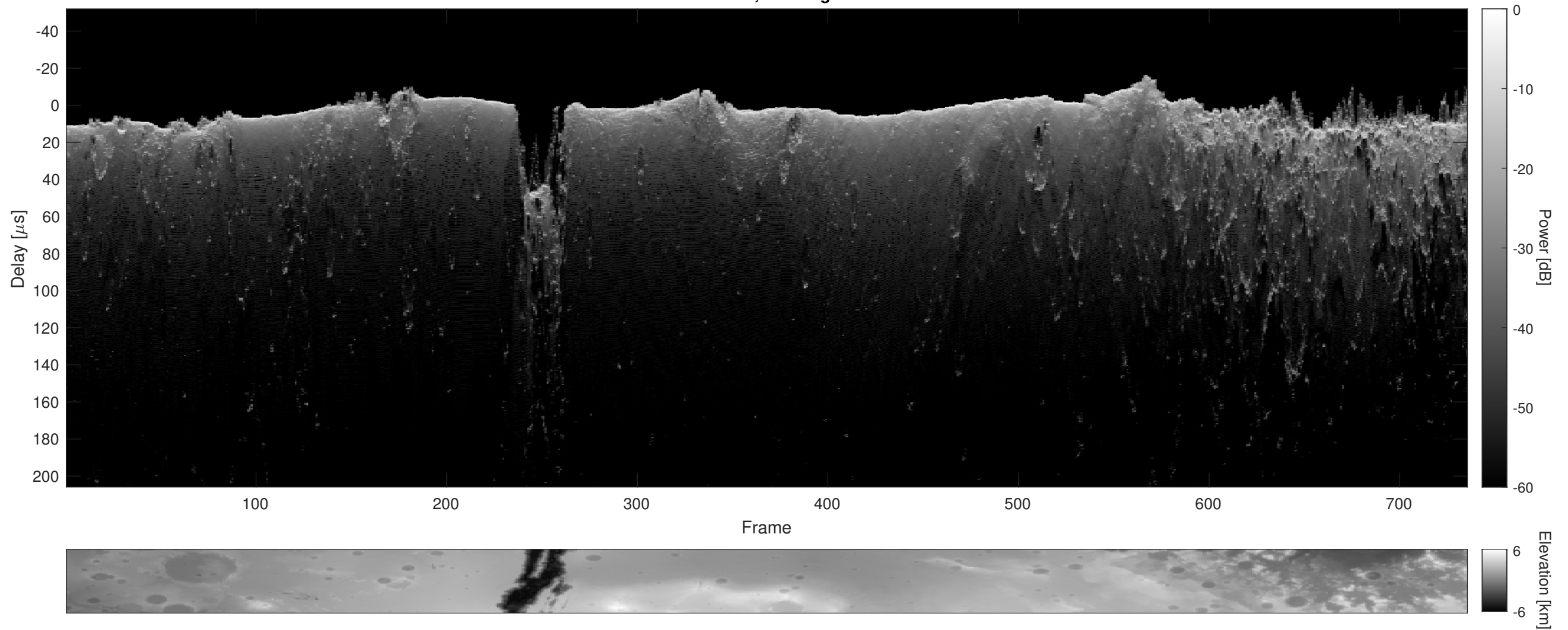
Orbit 3041, Cluttergram
