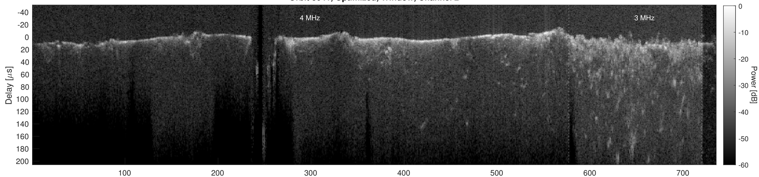
Orbit 3041, Cluttergram
