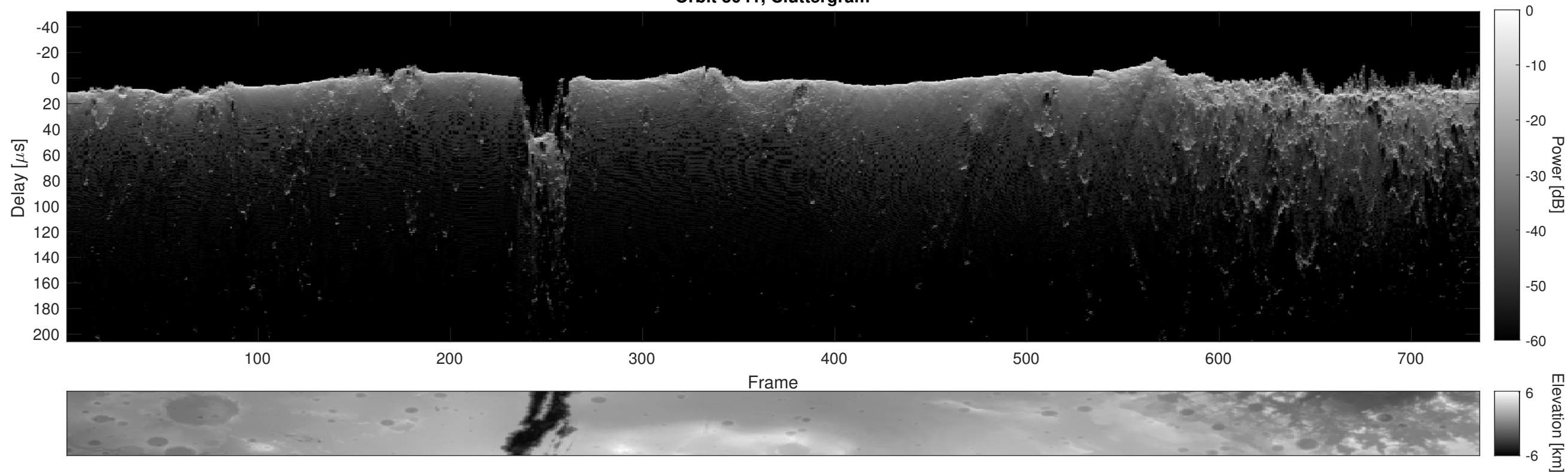
Orbit 3041, Cluttergram
