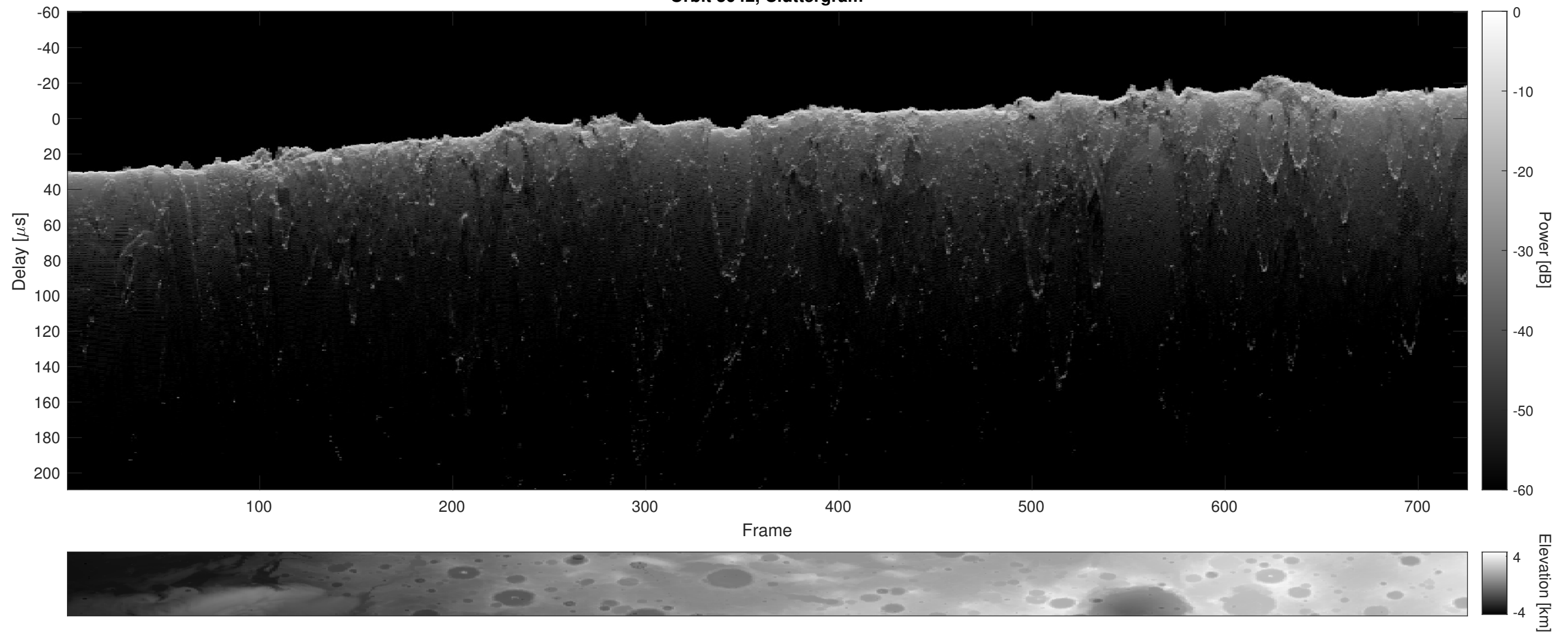
Orbit 3042, Cluttergram
