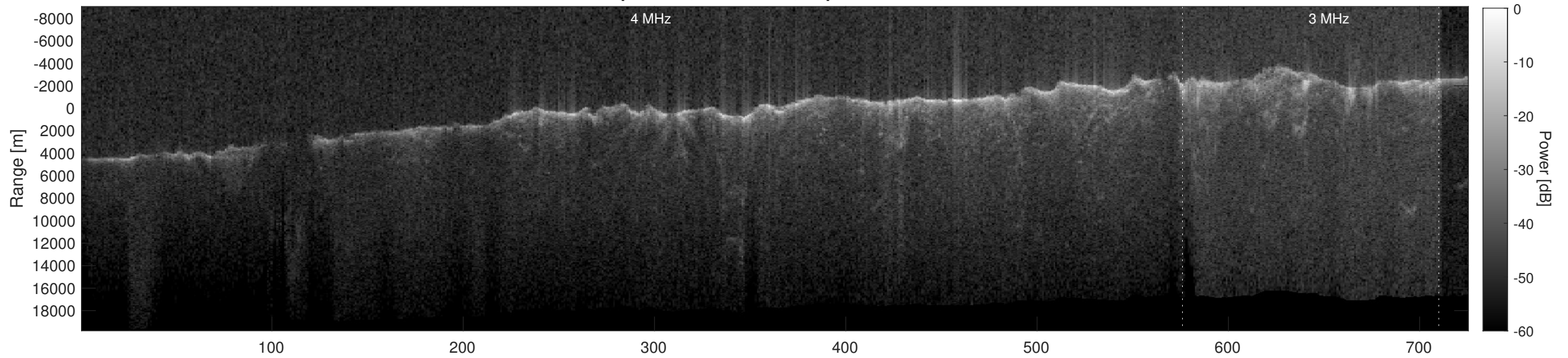
Orbit 3042, Depth-Corrected Cluttergram
