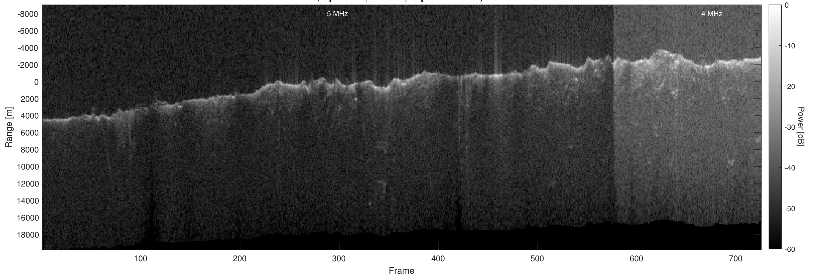
Orbit 3042, Optimized, Window, Depth-Corrected, Channel 2
