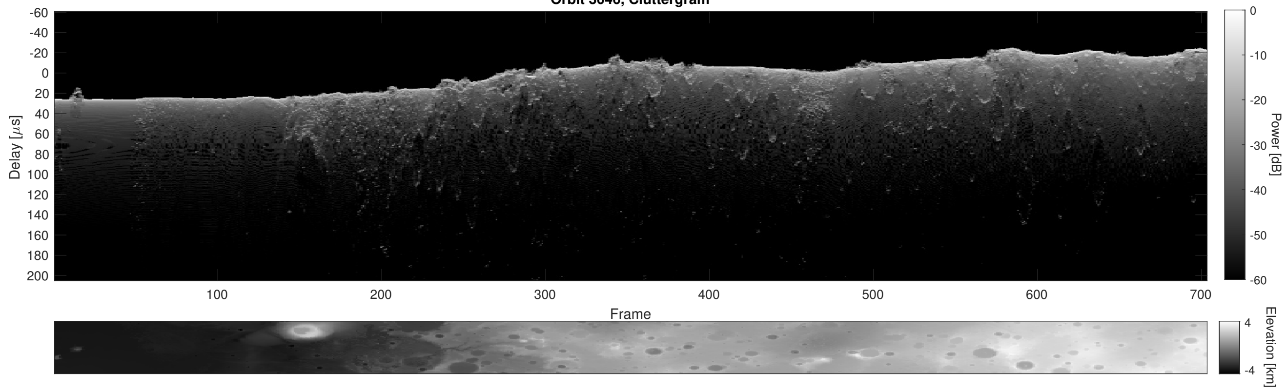
Orbit 3046, Cluttergram
