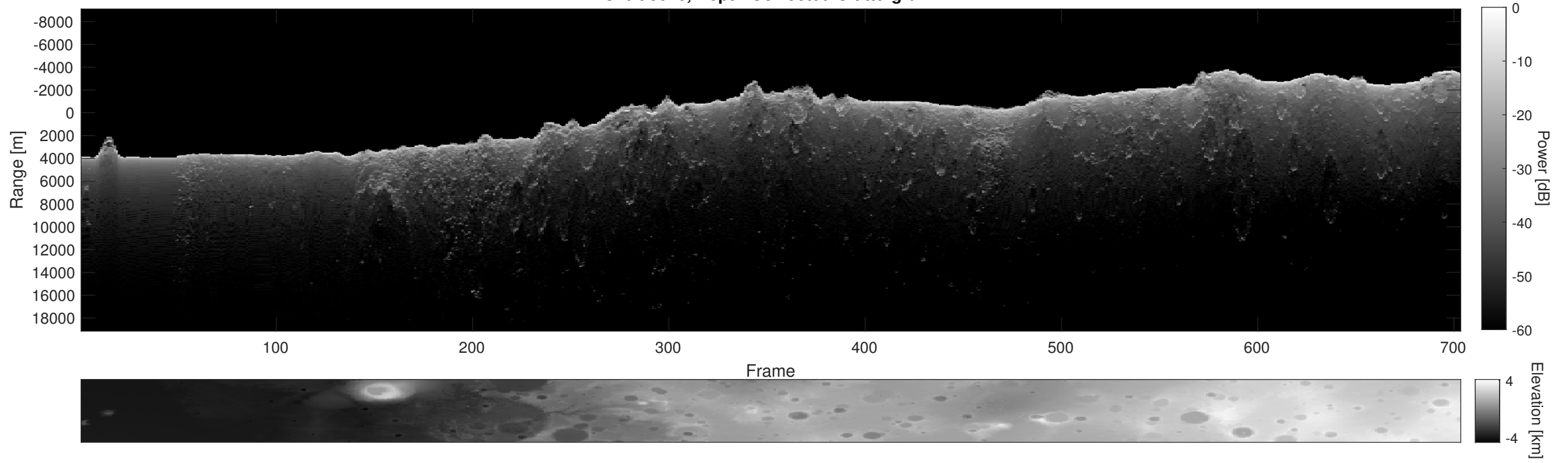
Orbit 3046, Depth-Corrected Cluttergram
