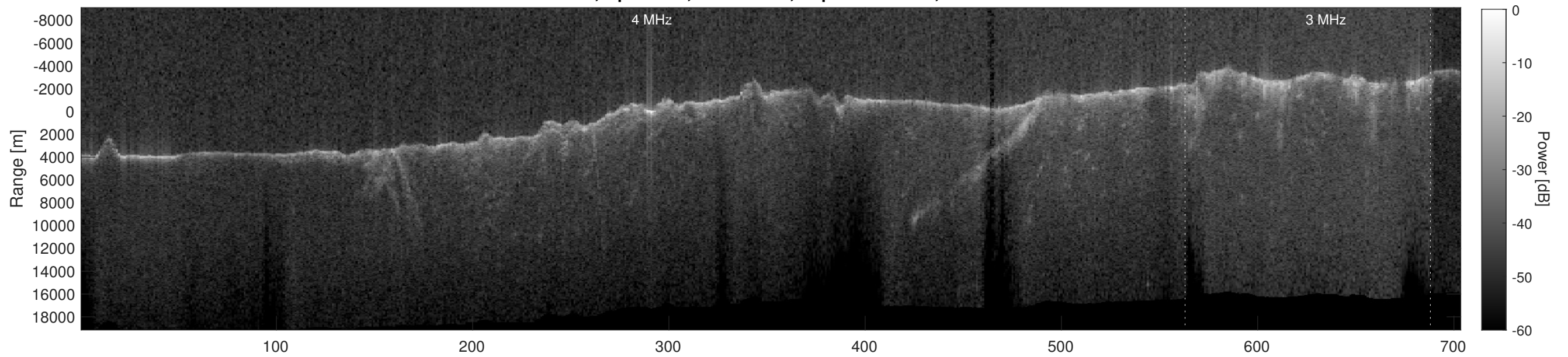
Orbit 3046, Depth-Corrected Cluttergram
