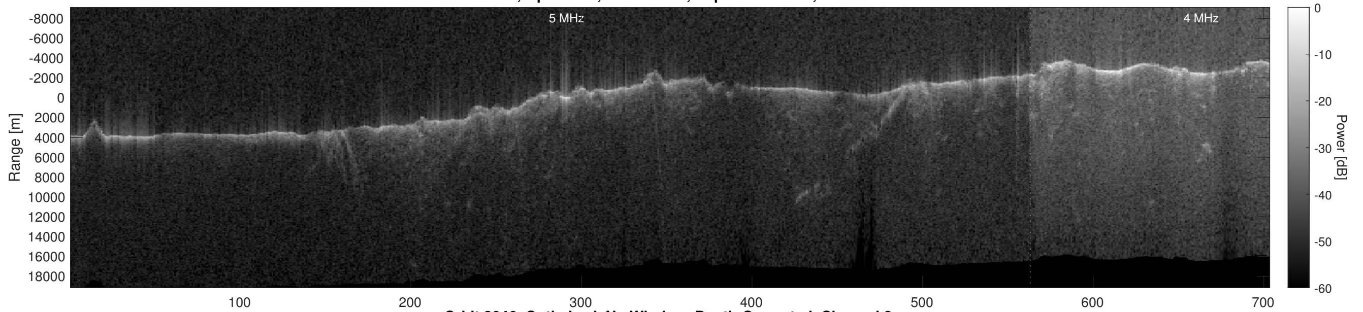
Orbit 3046, Optimized, No Window, Depth-Corrected, Channel 2
