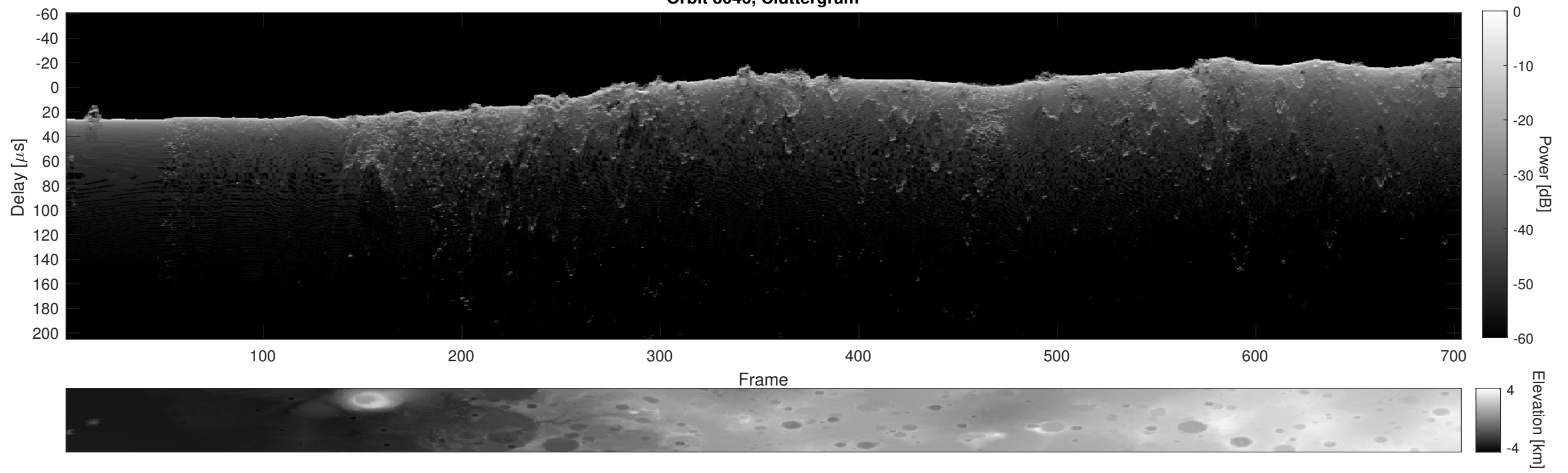
Orbit 3046, Cluttergram
