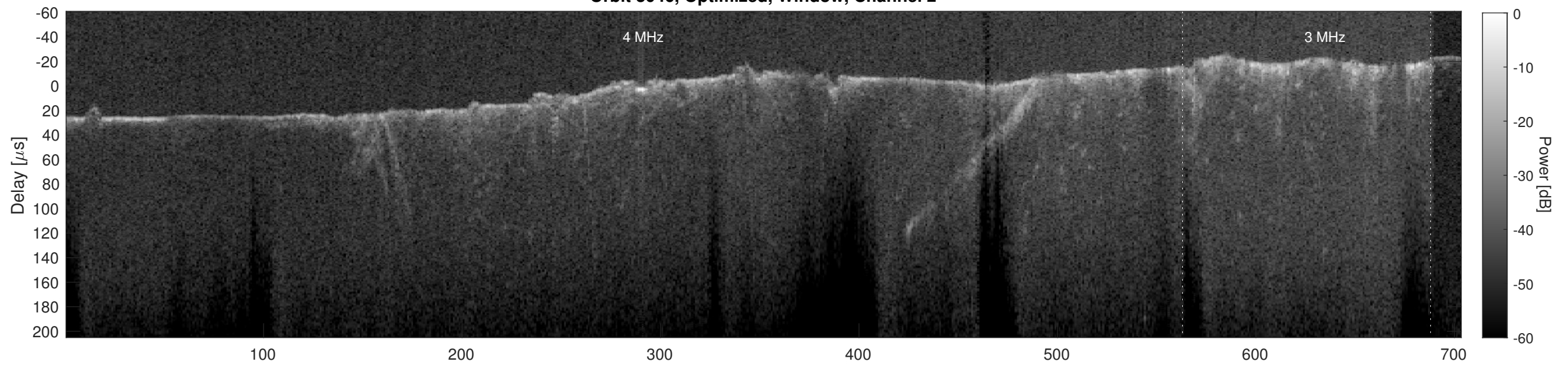
Orbit 3046, Cluttergram
