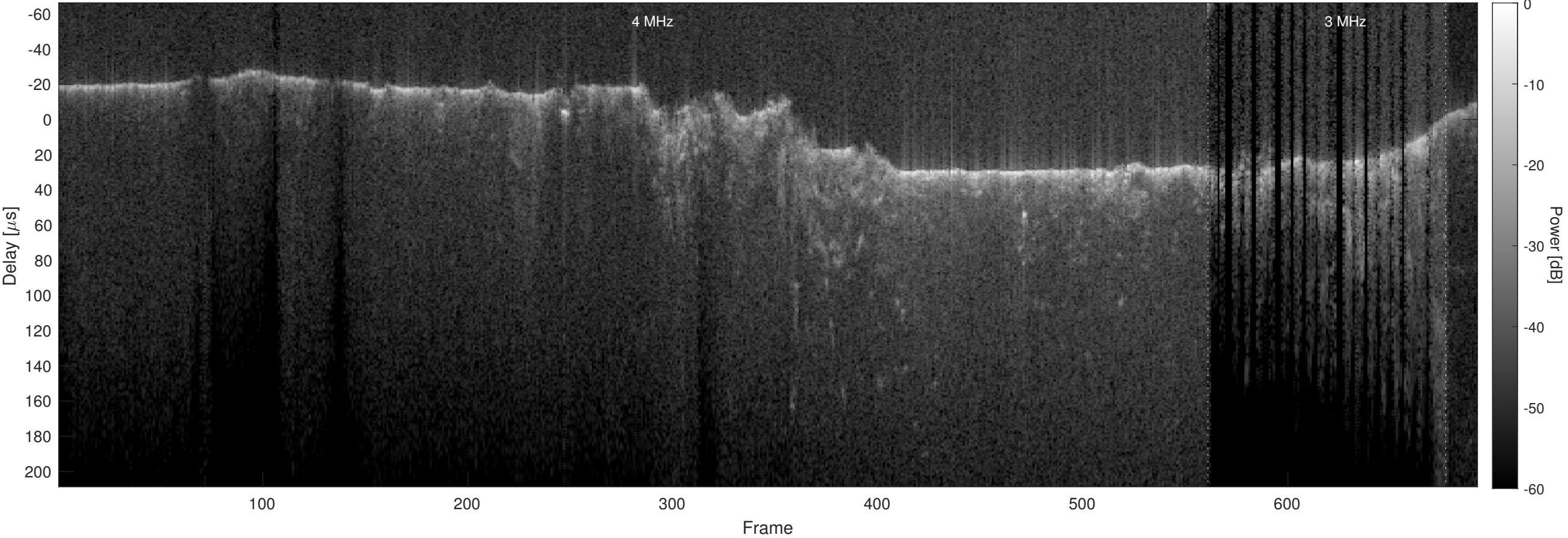
Orbit 3047, Optimized, No Window, Channel 2
