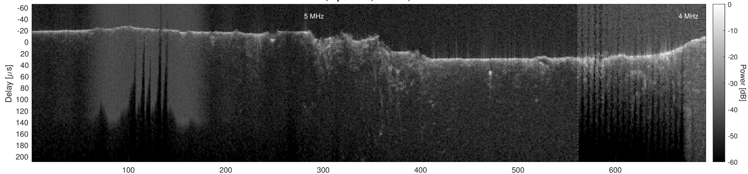
Orbit 3047, Optimized, Window, Channel 2
