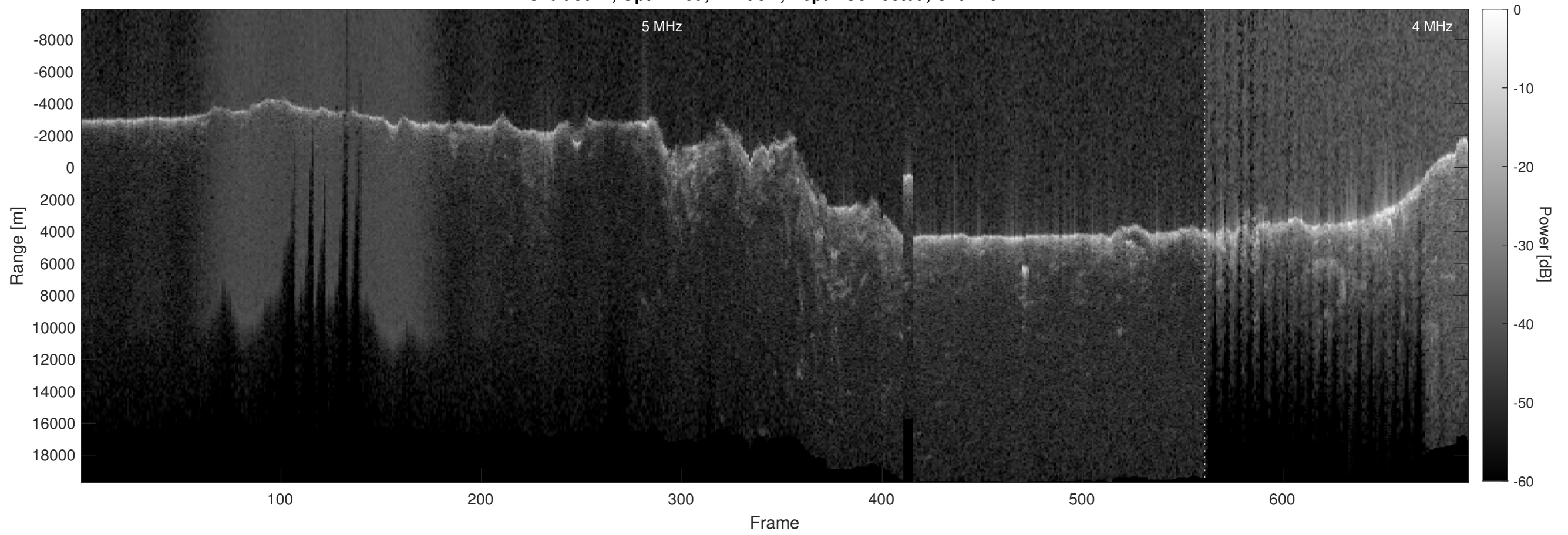
Orbit 3047, Optimized, Window, Depth-Corrected, Channel 2
