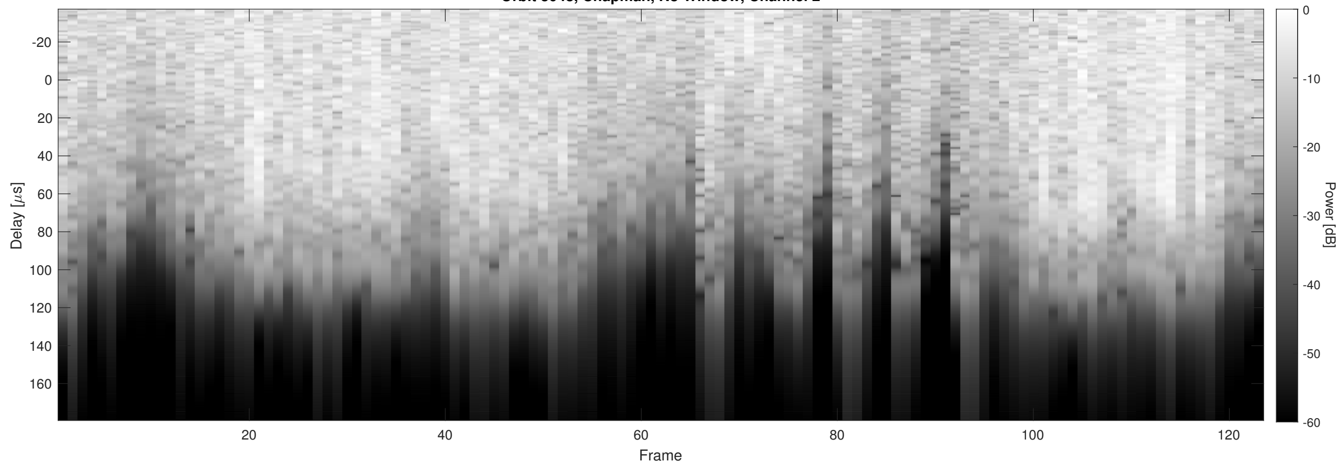
Orbit 3048, Chapman, No Window, Channel 2
