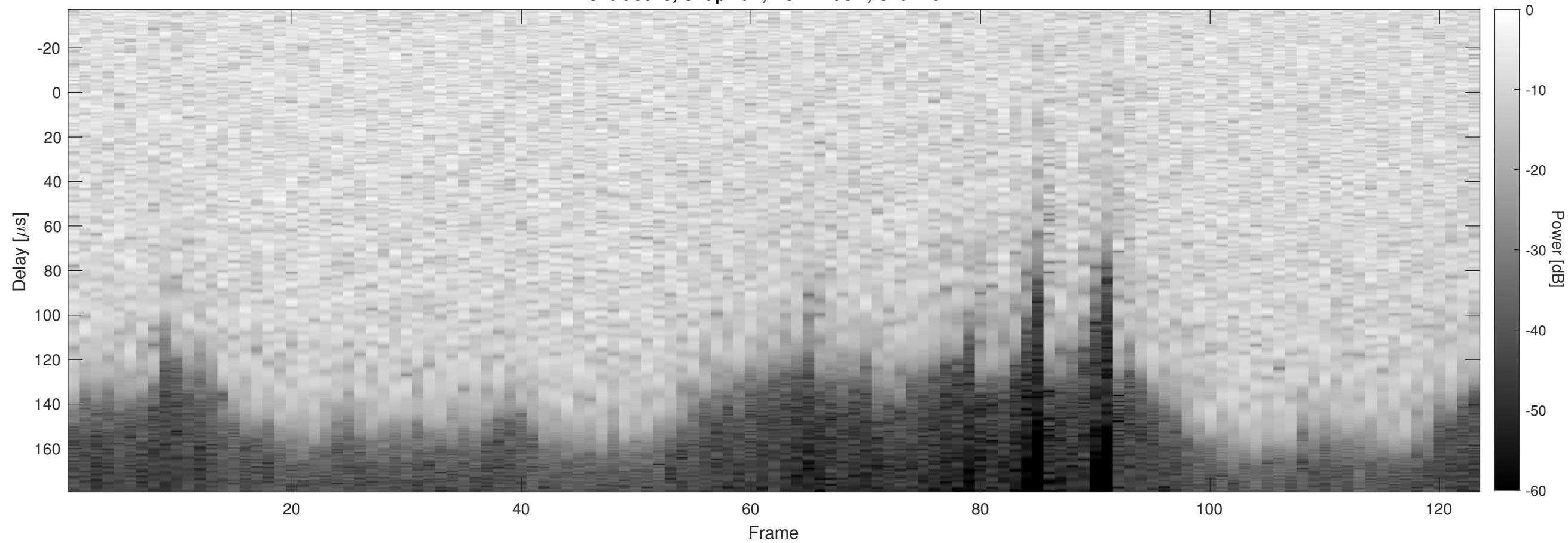
Orbit 3048, Chapman, No Window, Channel 2
