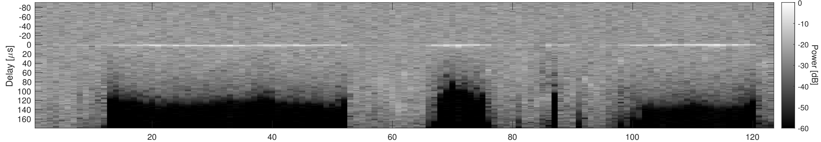
Orbit 3048, Cluttergram
