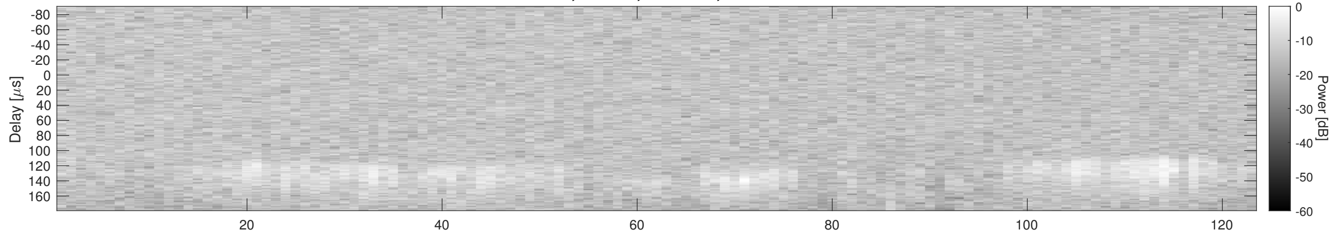
Orbit 3048, Window, Channel 2, Chapman
