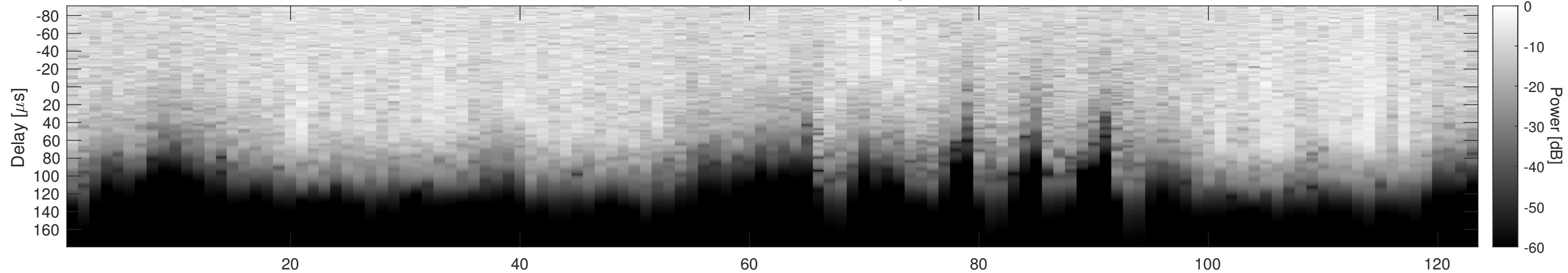
Orbit 3048, Window, Channel 2, Optimized
