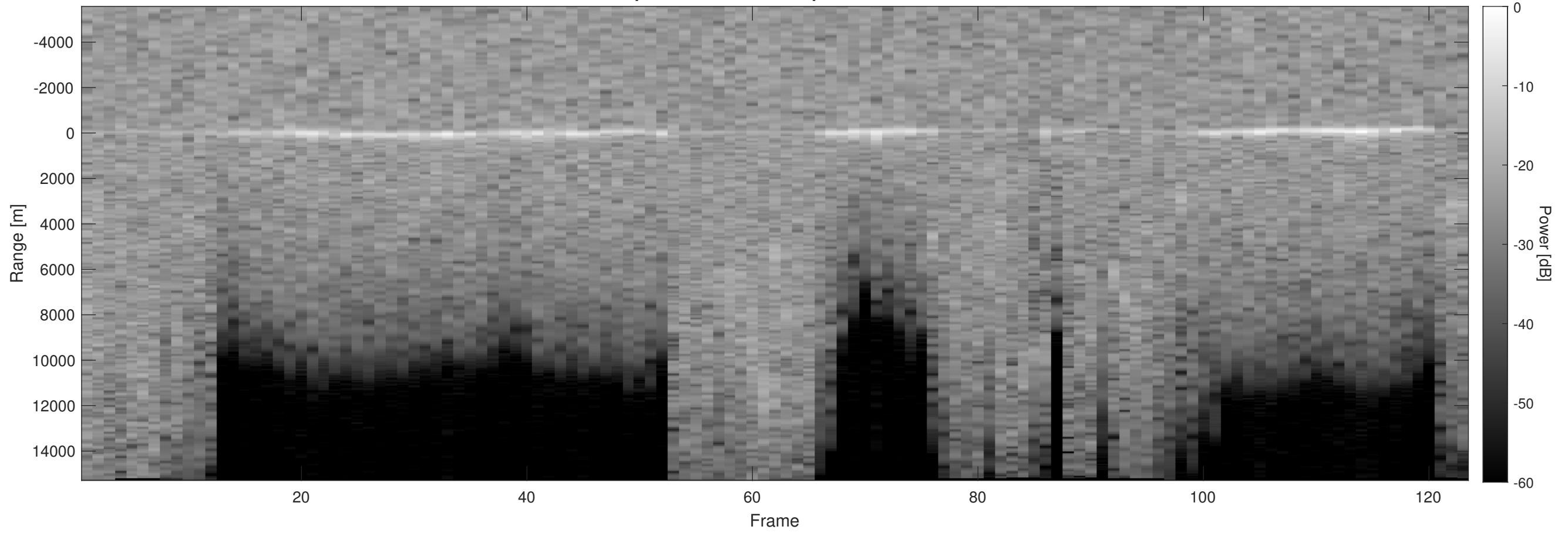
Orbit 3048, Optimized, Window, Depth-Corrected, Channel 2
