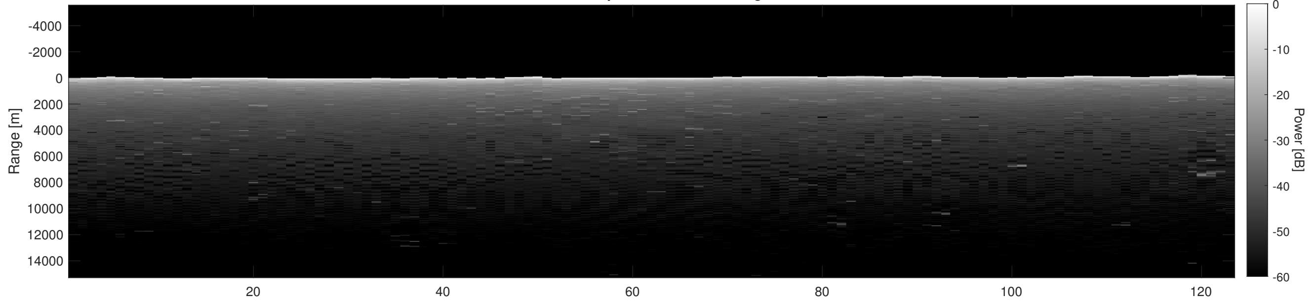
Orbit 3048, Depth-Corrected Cluttergram
