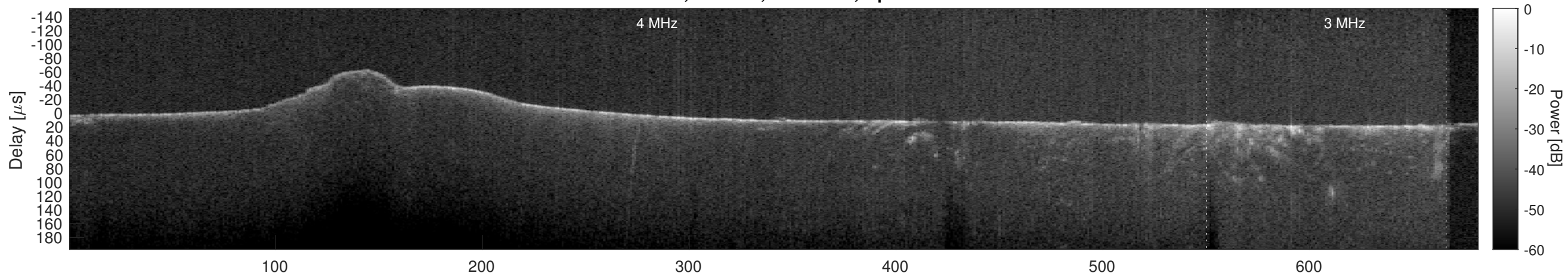
Orbit 3049, Cluttergram
