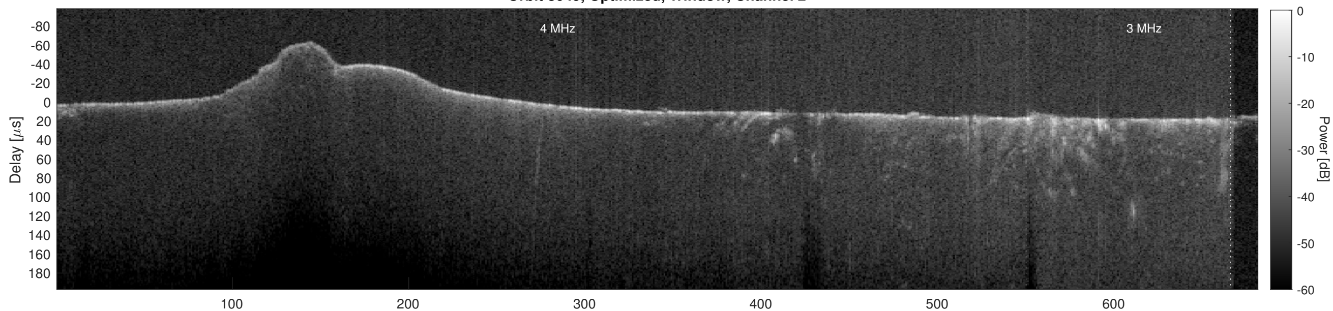
Orbit 3049, Cluttergram
