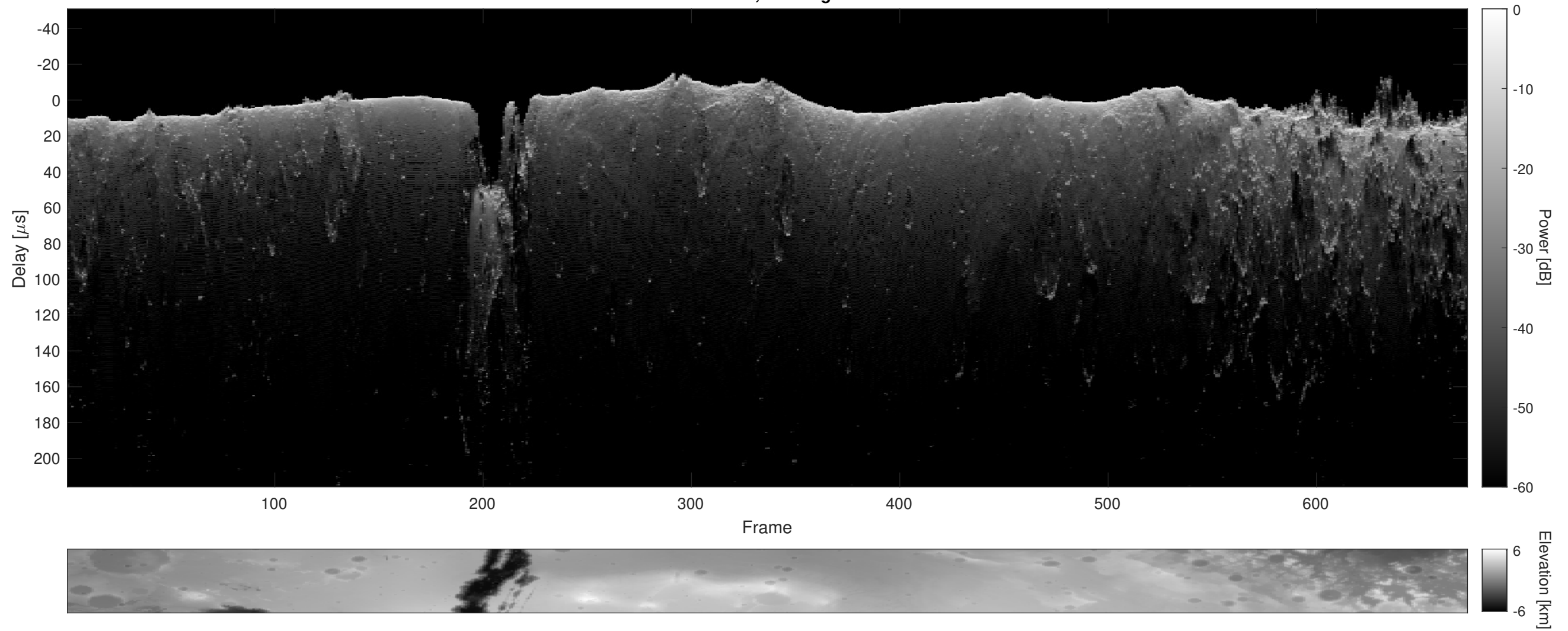
Orbit 3052, Cluttergram
