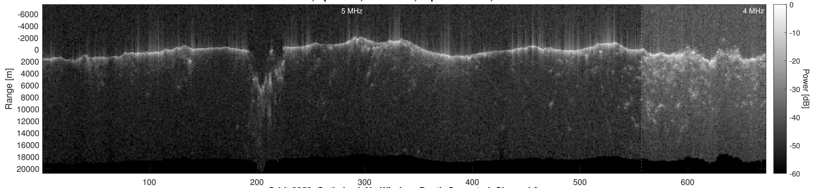
Orbit 3052, Optimized, No Window, Depth-Corrected, Channel 2
