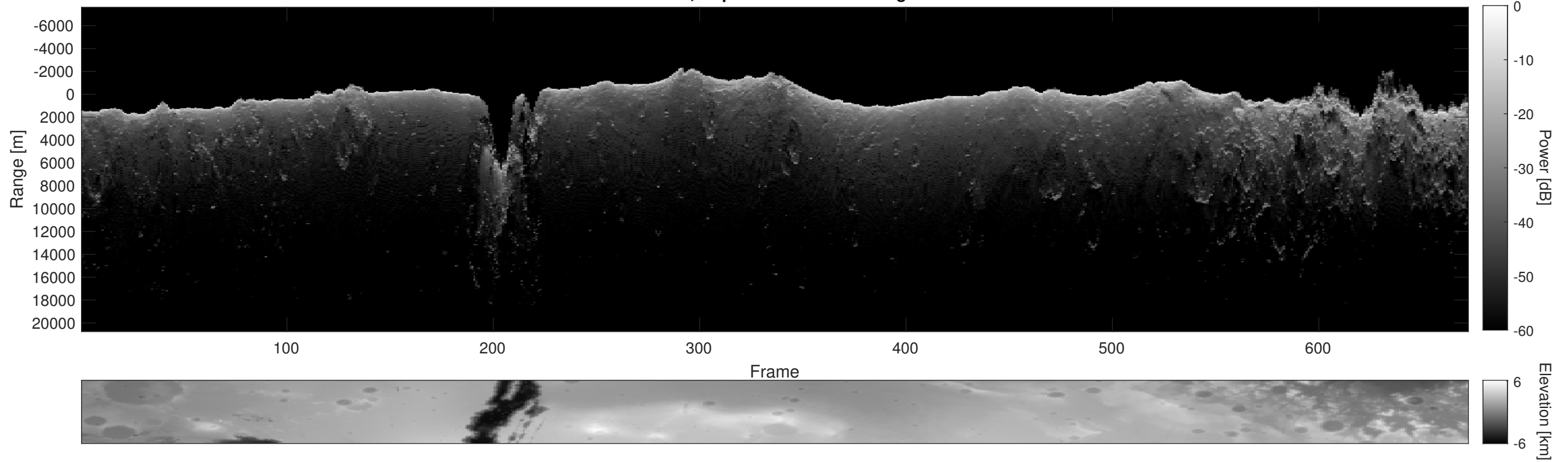
Orbit 3052, Depth-Corrected Cluttergram
