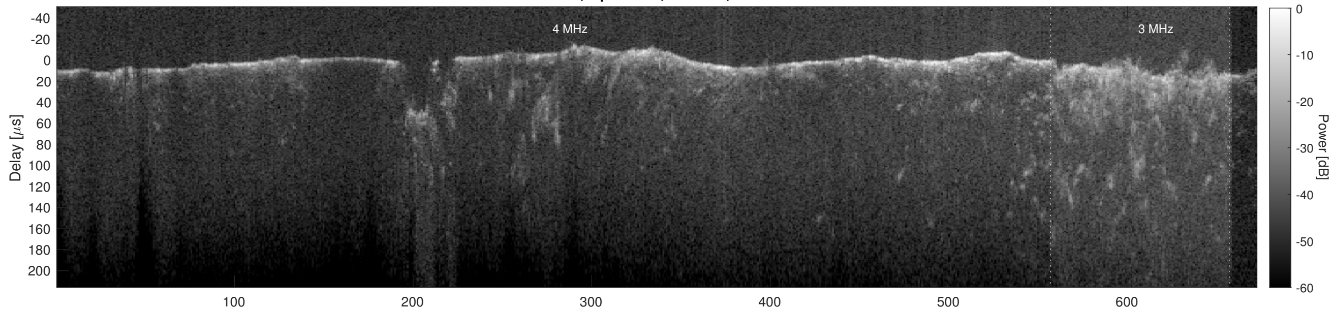
Orbit 3052, Cluttergram
