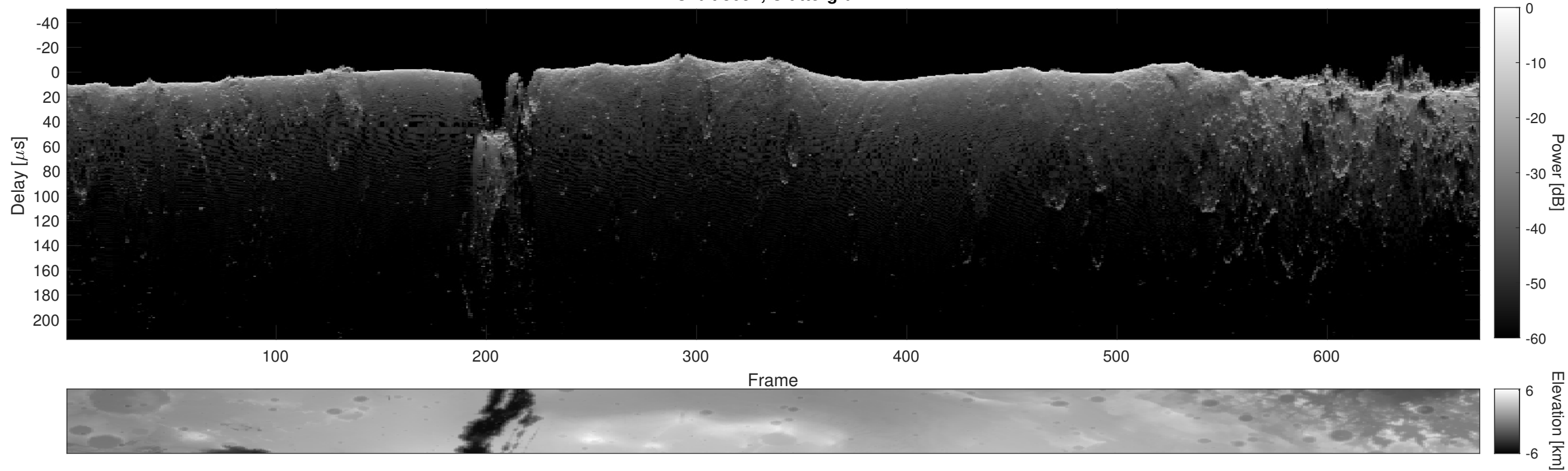
Orbit 3052, Cluttergram
