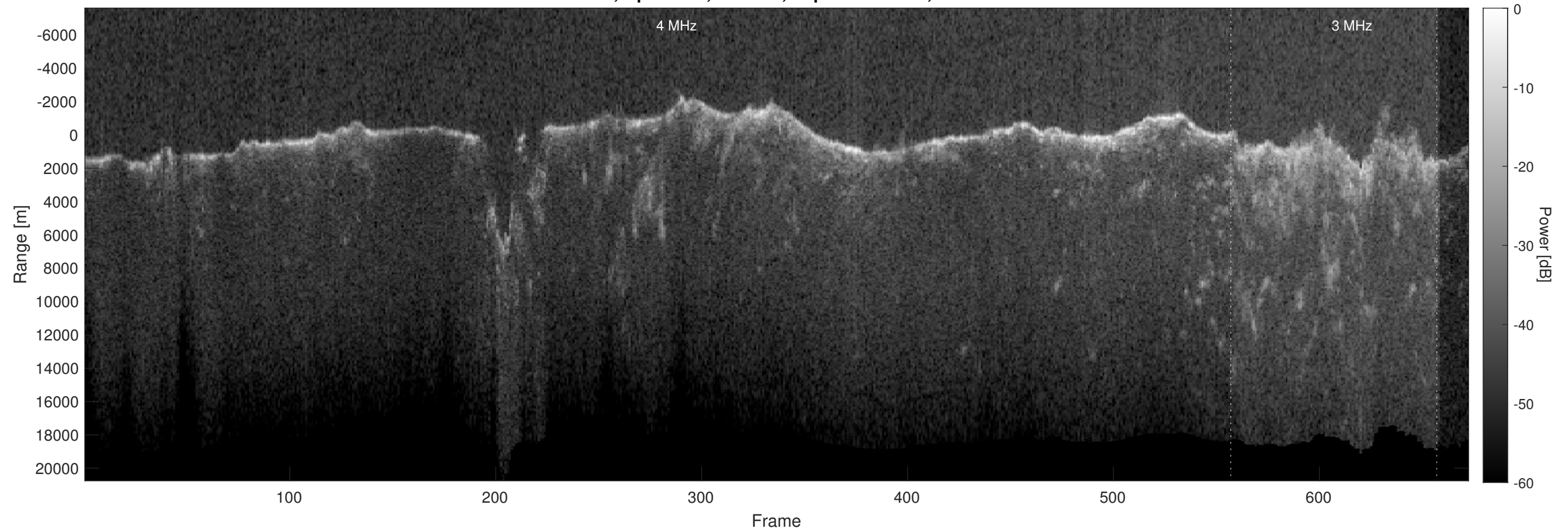
Orbit 3052, Optimized, Window, Depth-Corrected, Channel 2
