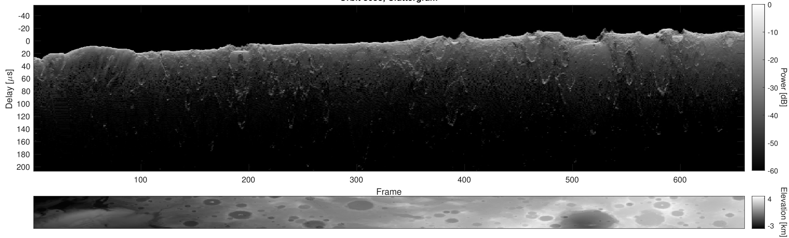
Orbit 3053, Cluttergram
