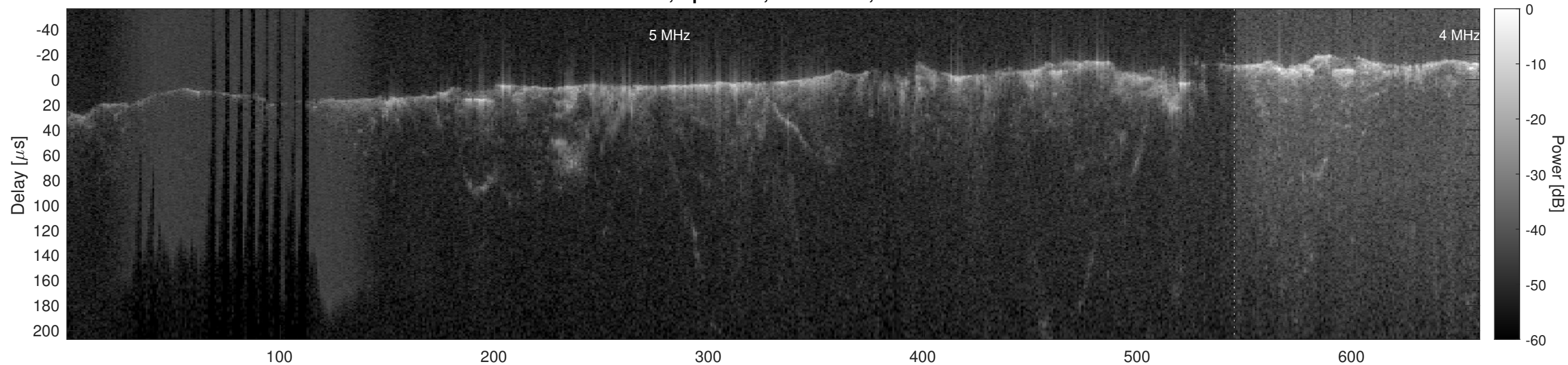
Orbit 3053, Optimized, No Window, Channel 2
