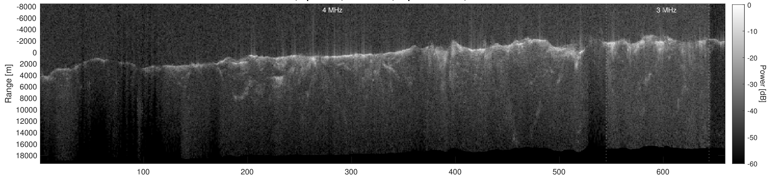
Orbit 3053, Depth-Corrected Cluttergram
