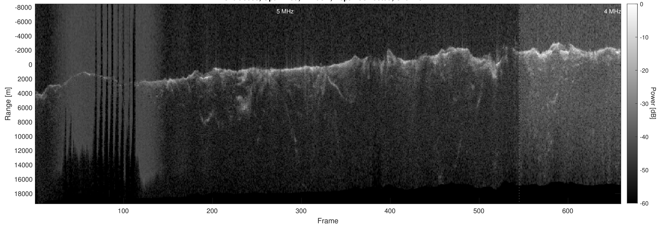
Orbit 3053, Optimized, Window, Depth-Corrected, Channel 2
