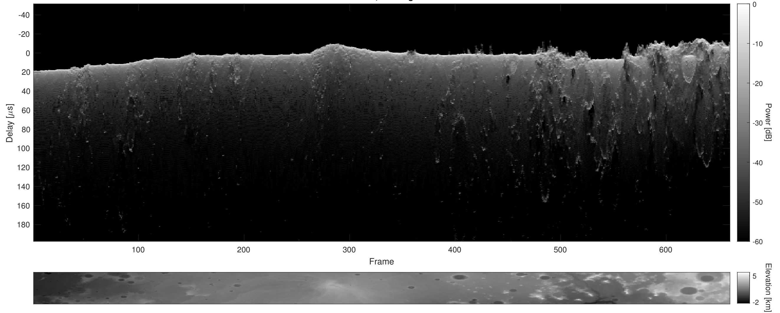
Orbit 3054, Cluttergram
