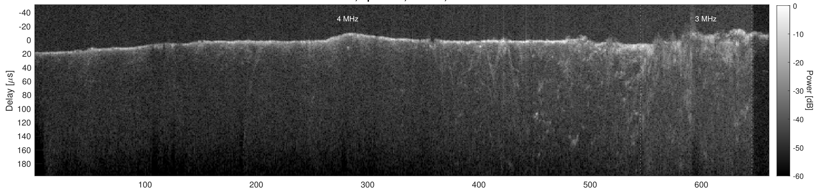
Orbit 3054, Cluttergram
