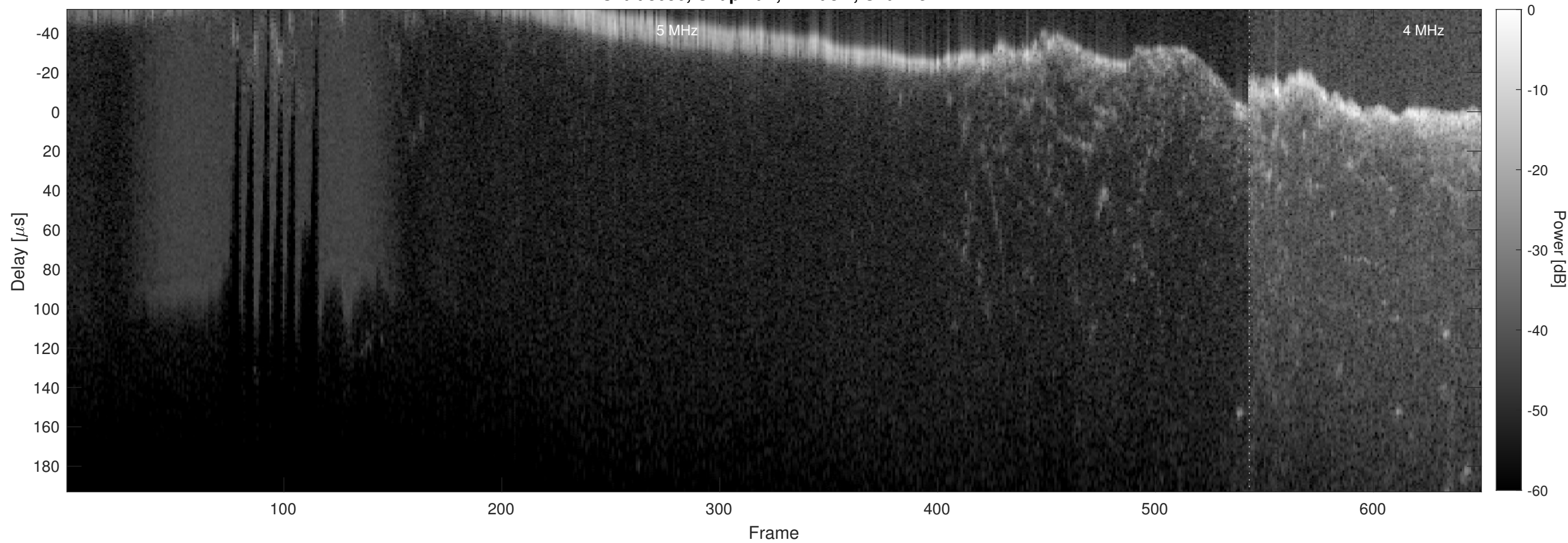
Orbit 3056, Chapman, Window, Channel 2
