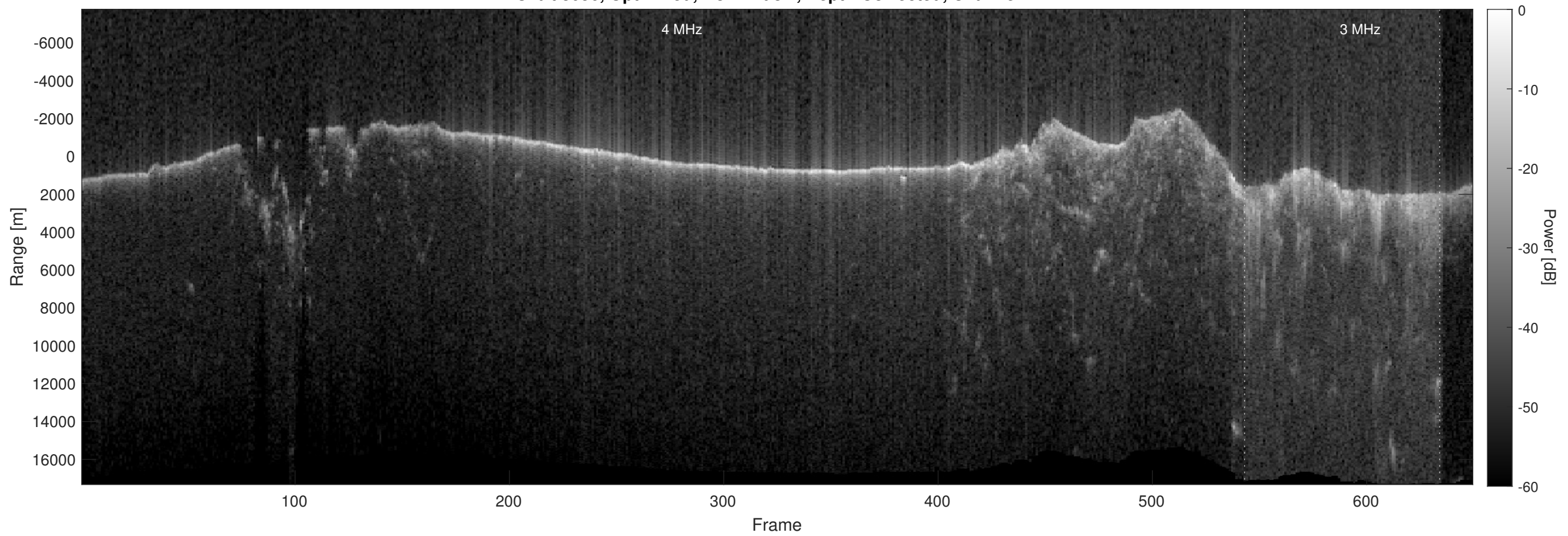
Orbit 3056, Optimized, No Window, Depth-Corrected, Channel 2
