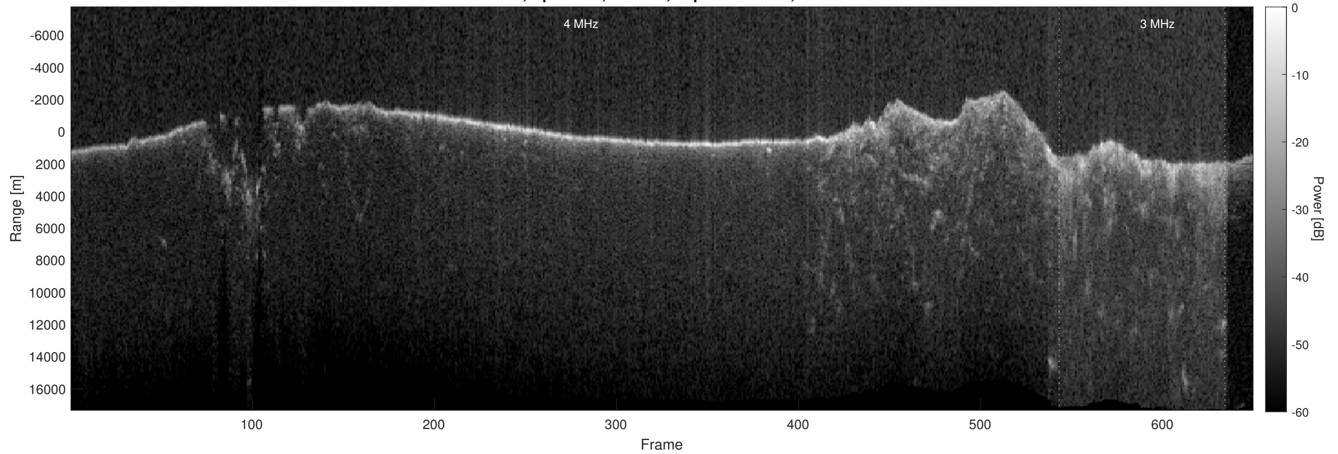
Orbit 3056, Optimized, Window, Depth-Corrected, Channel 2
