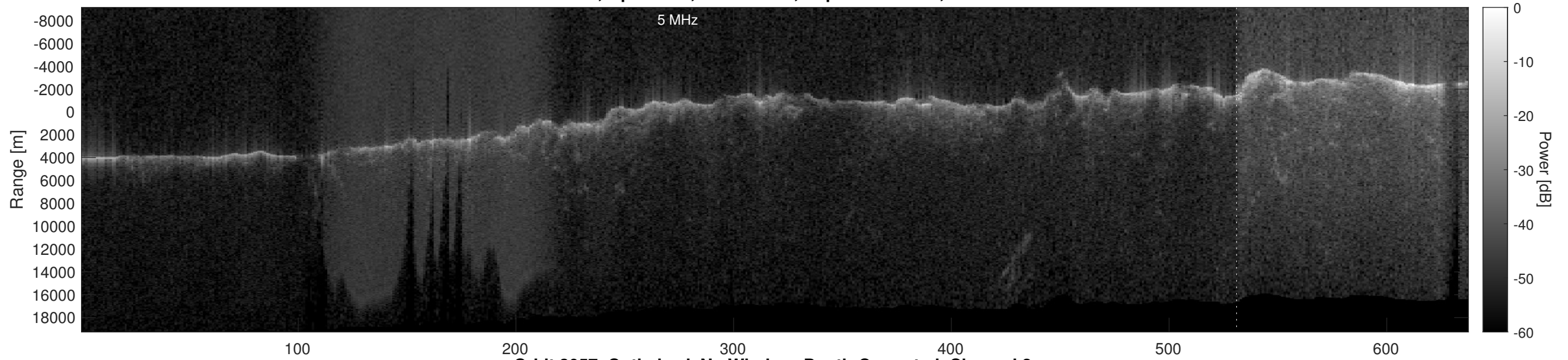
Orbit 3057, Optimized, No Window, Depth-Corrected, Channel 2
