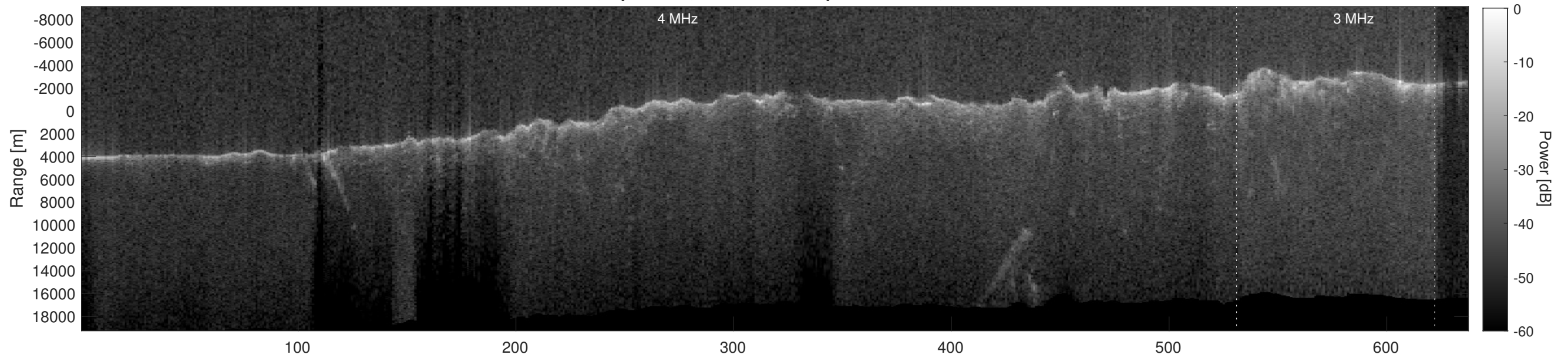
Orbit 3057, Depth-Corrected Cluttergram
