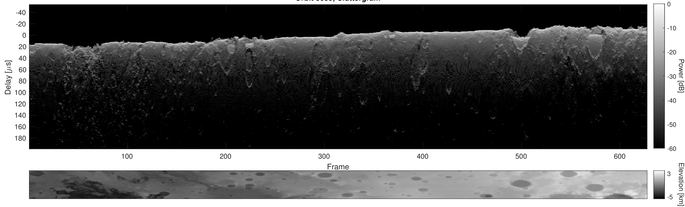
Orbit 3059, Cluttergram
