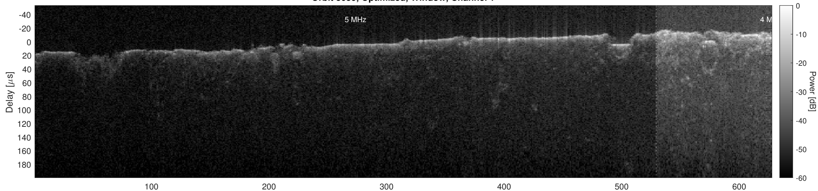
Orbit 3059, Optimized, Window, Channel 2
