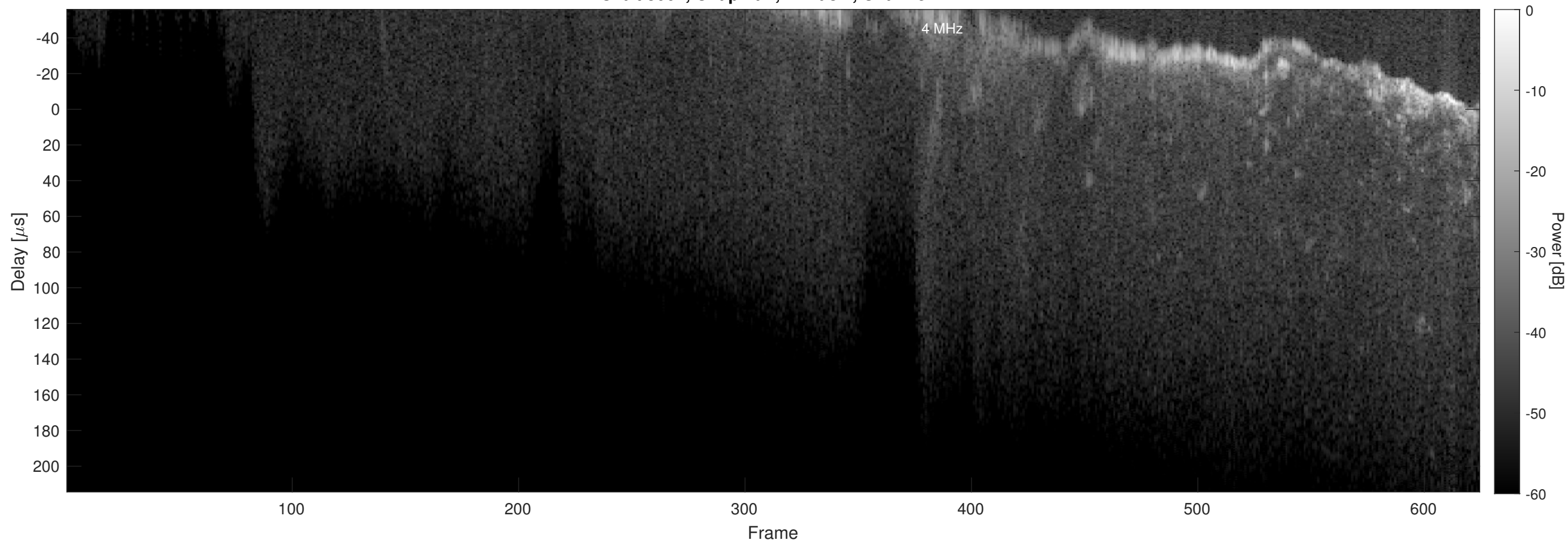
Orbit 3061, Chapman, Window, Channel 2
