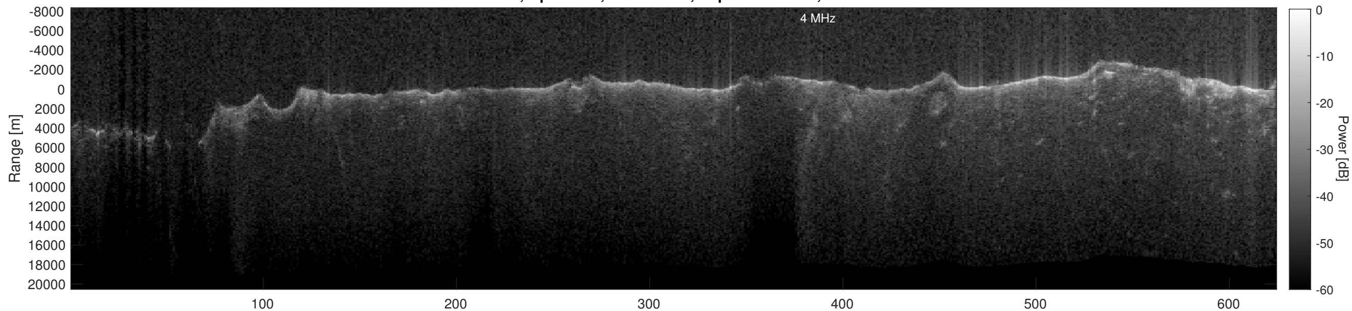
Orbit 3061, Depth-Corrected Cluttergram
