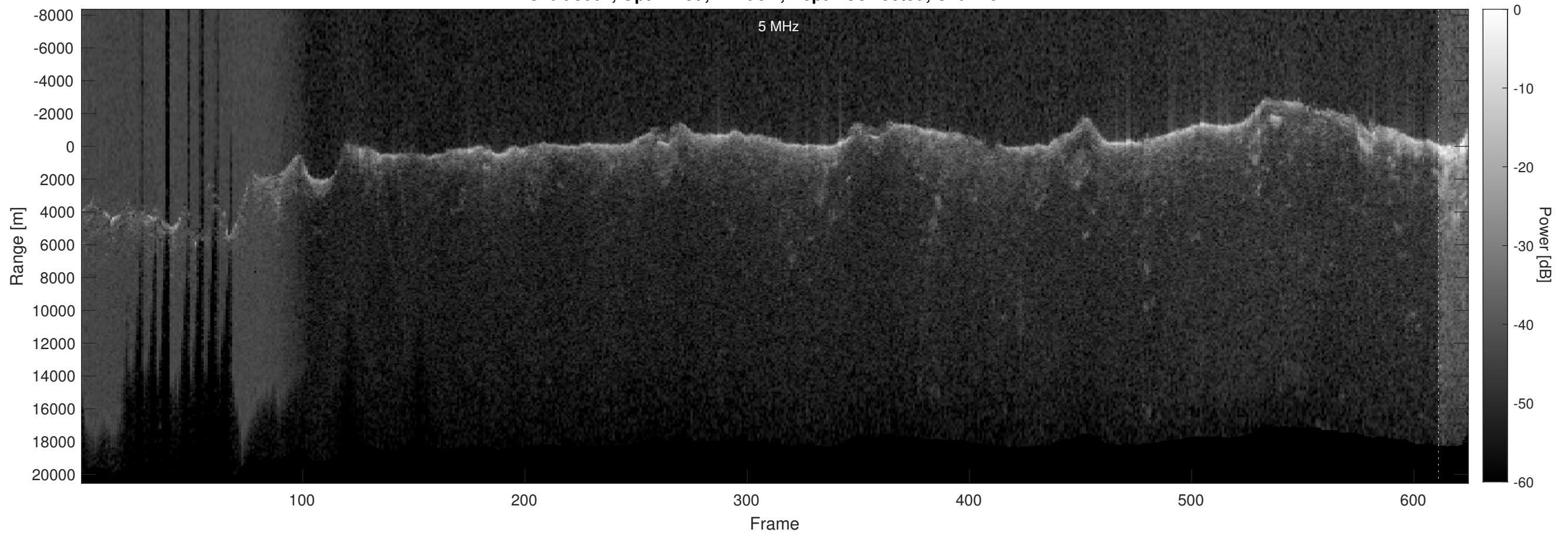
Orbit 3061, Optimized, Window, Depth-Corrected, Channel 2
