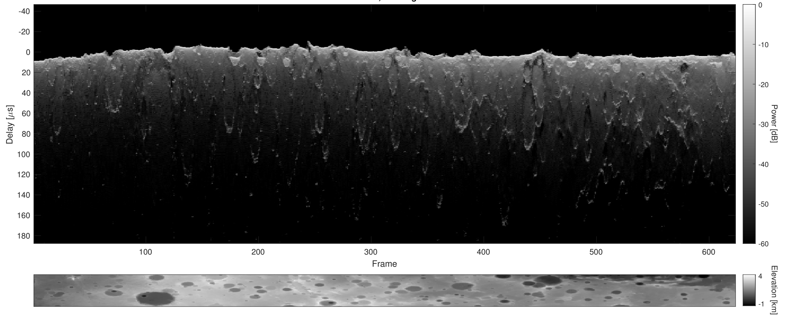
Orbit 3062, Cluttergram
