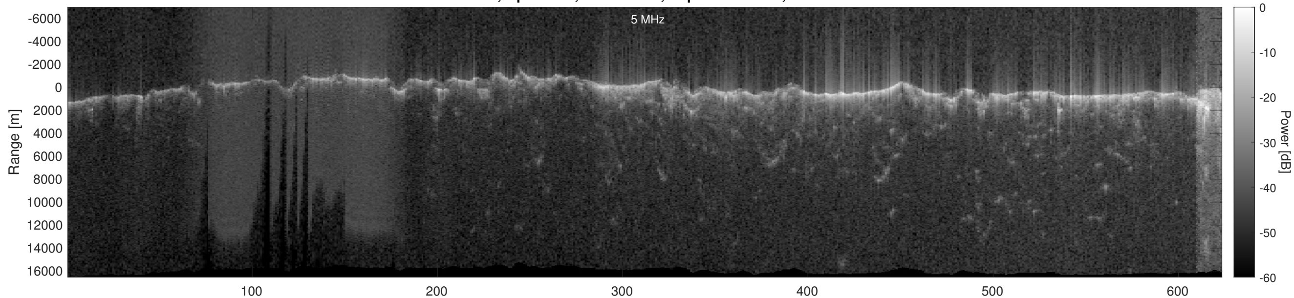
Orbit 3062, Optimized, No Window, Depth-Corrected, Channel 2
