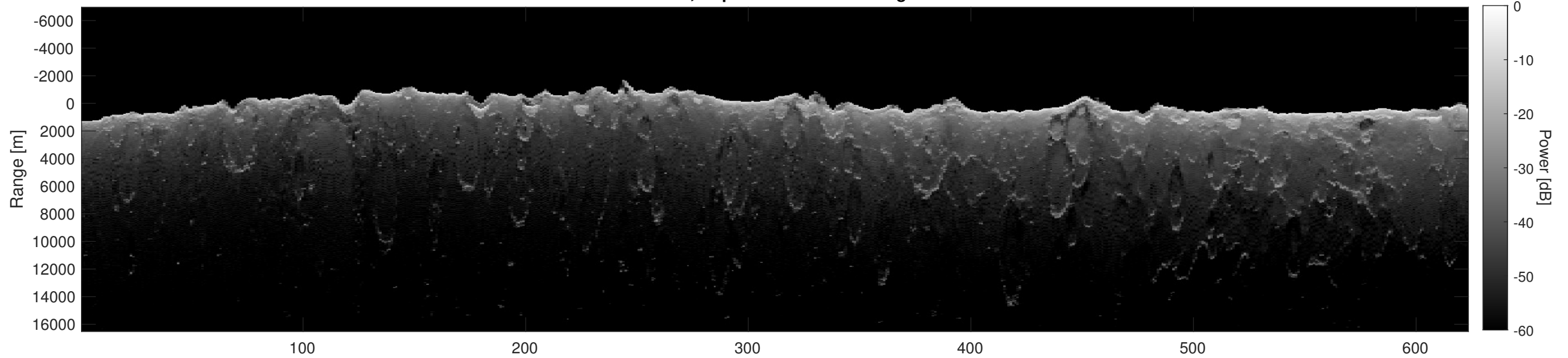
Orbit 3062, Depth-Corrected Cluttergram
